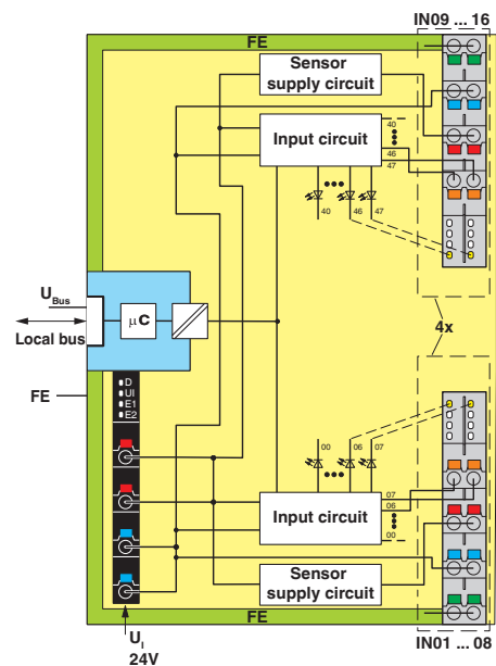
Block diagram
